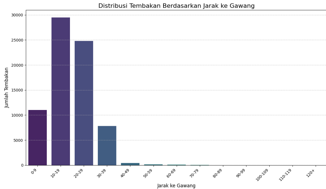
Gambar 4.22 Visualisasi Distribusi Fitur distance_to_goal
