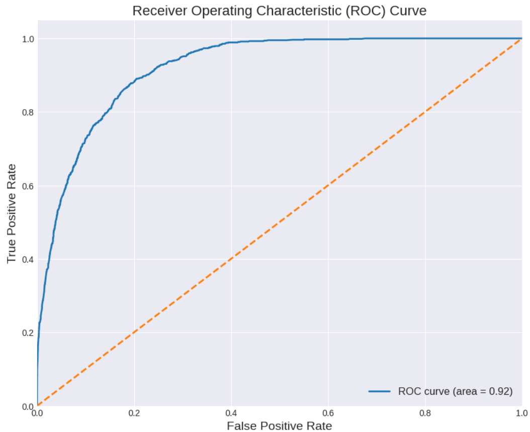
Gambar 4.29 Receiver Operating Characteristic (ROC) Curve
