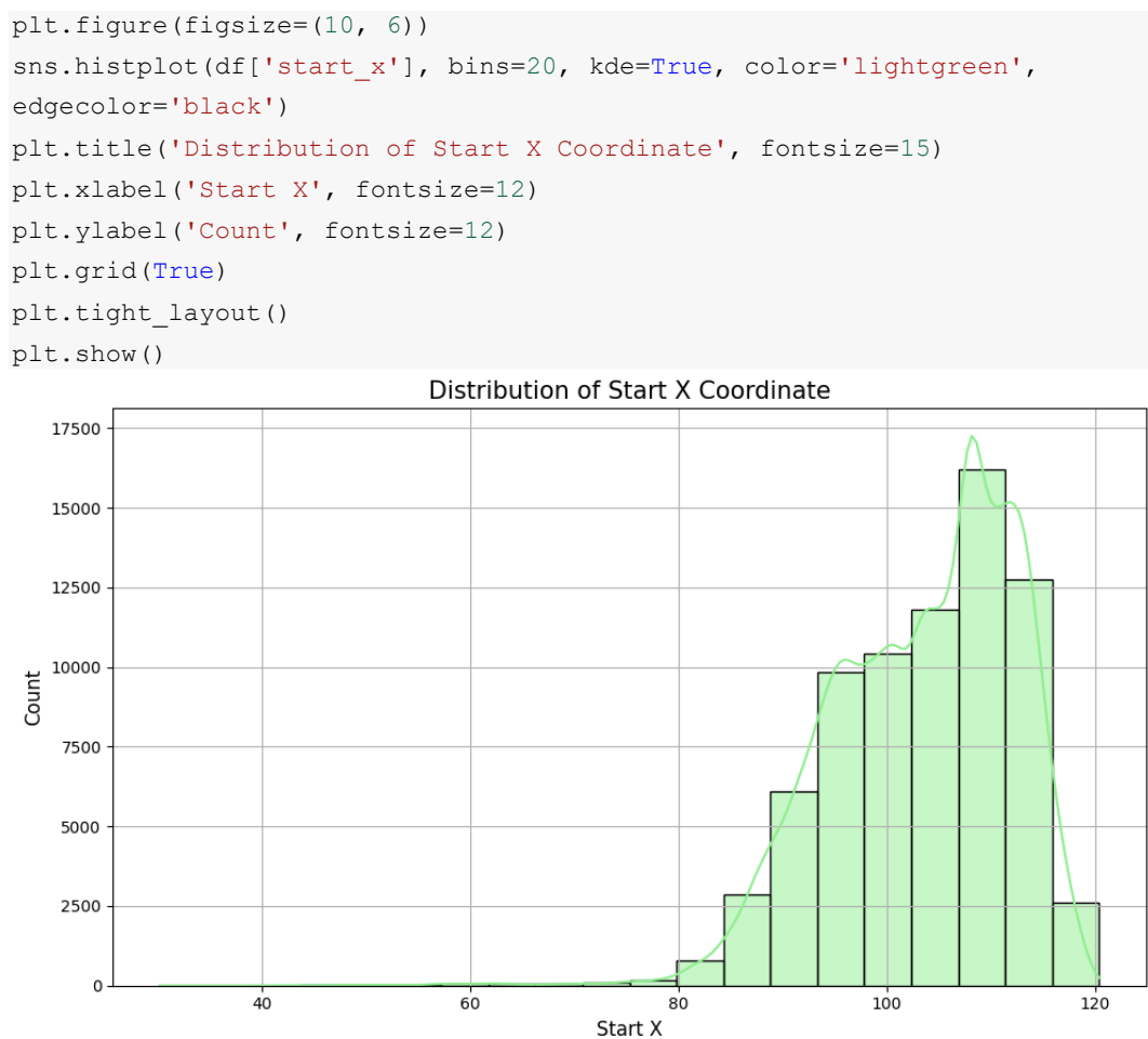
Gambar 4.10 Distribusi Koordinat Start x
